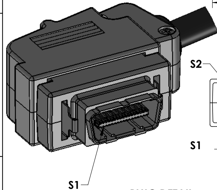
PLUG DETAIL SCALE 2:1
