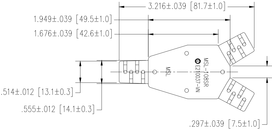
JUNCTION P4 BACK VIEW
