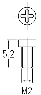
M2 Screw
