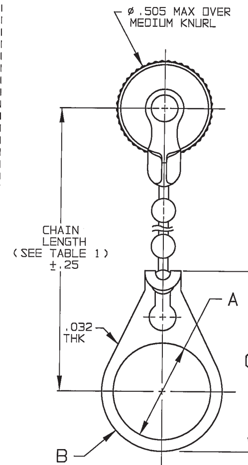
-2-D2 THRU -11-DD8 SHOWN STANDARD CHAIN AND BULKHEAD JACK MOUNTING LUG
