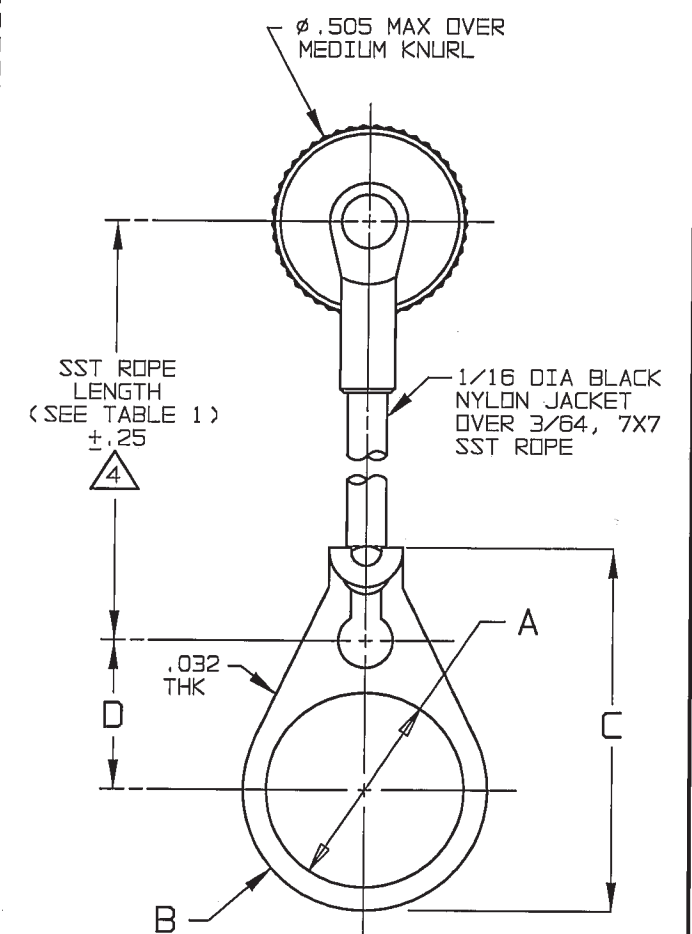
-12-D2 THRU -17-DD8 SHOWN STAINLESS STEEL ROPE AND BULKHEAD JACK MOUNTING LUG
