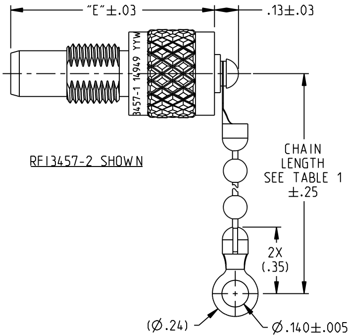
RFIX457XX-2 THRU RFI457XX-11 BEAD CHAIN & END RING
