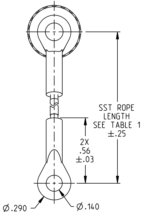
RFIX457XX-12 THRU RFI457XX-17 SST ROPE & MTG LUG
