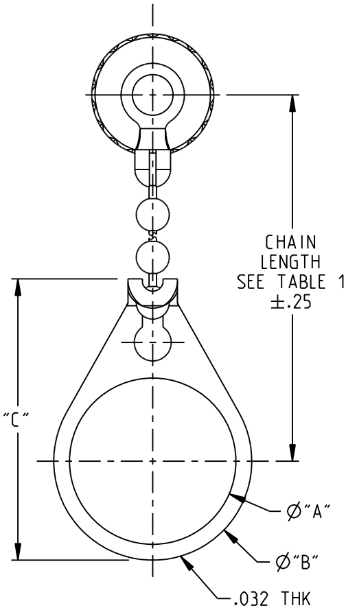
RFIX457XX-2-D2 THRU RFI457XX-11-DD8 BEAD CHAIN w/BULKHEAD MTG LUG
