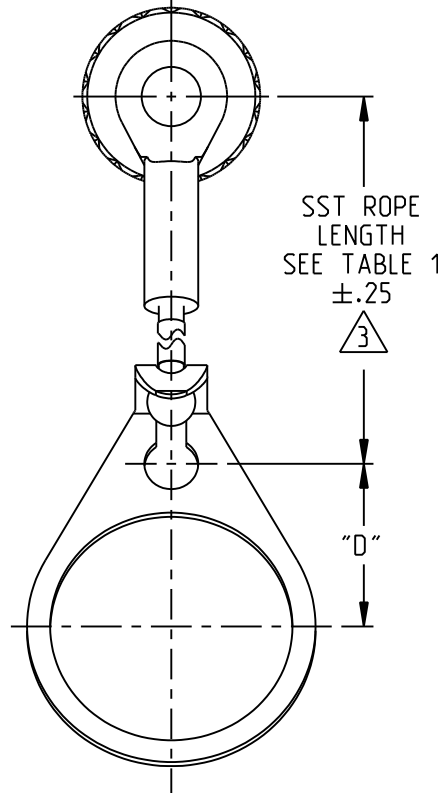
RFIX457XX-12-D2 THRU RFIX457XX-17-DD8 SST ROPE w/BULKHEAD MTG LUG
