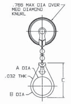
RFI85/RFI853-2-01 THRU -11-008 SHOWN STANDARD CHAIN AND BULKHEAD JACK MOUNTING LUG
