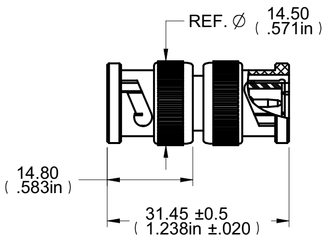
DIM OUTLINE
