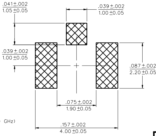
RECOMMENDED PCB PATTERN
