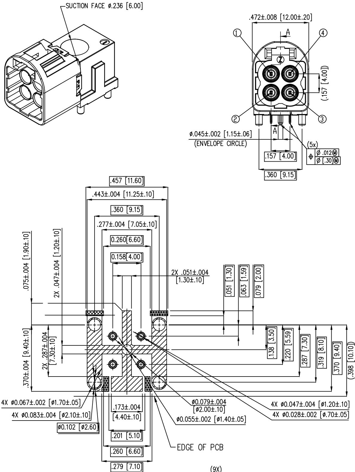
RECOMMENDED PCB LAYOUT
