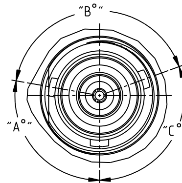
KEYING DETAIL
