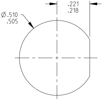
RECOMMENED PANEL CUTOUT
