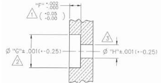
Recommended Mounting Hole Detail
